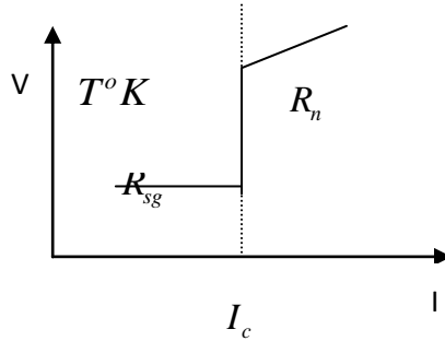
Figure-3. I-V characteristics of the junction
