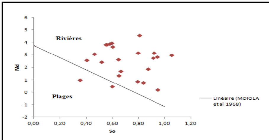
Figure 7 : Diagramme Md-So(MOIOLA and WEISER, 1968)
