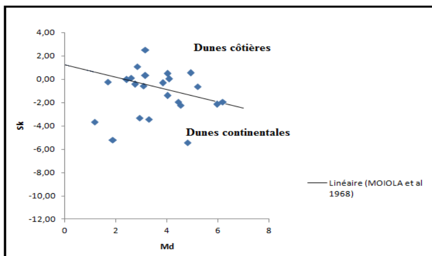
Figure 8 : Diagramme Sk-Md (MOIOLA and WEISER, 1968)
