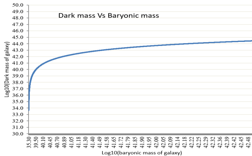
Figure 1. Galactic baryonic mass Vs Dark mass.
