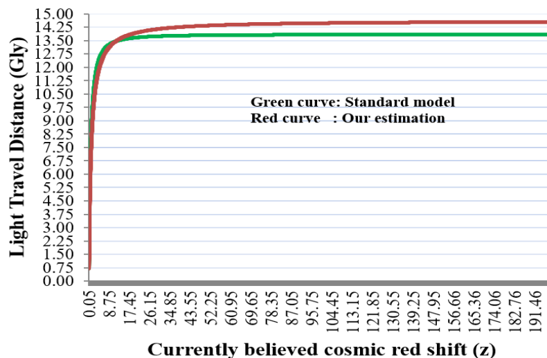
Figure 3. Comparison of standard and estimated light travel distances.
