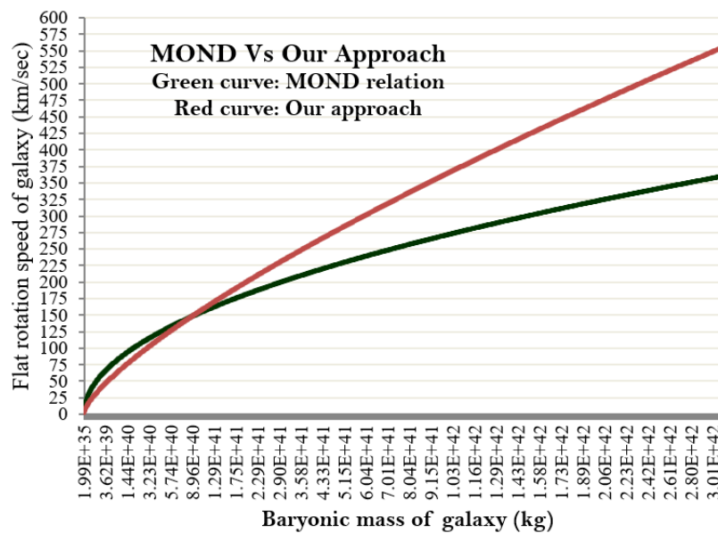
Figure 2. Galactic flat rotation speeds.
