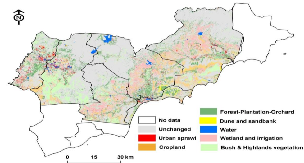
Fig-4 Change detection map for the studied area (spatial extends of converted classes are highlighted).
