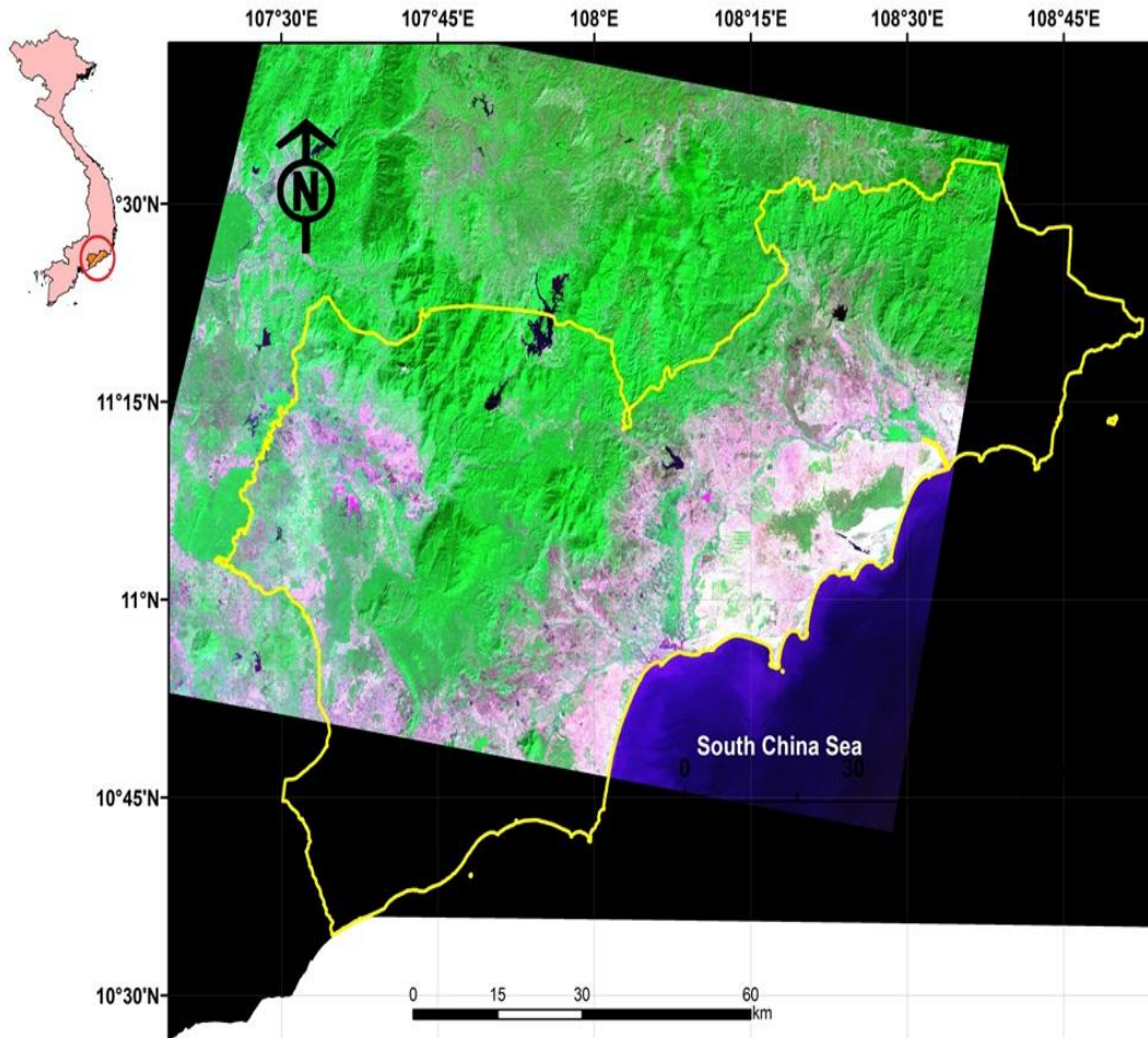
Fig-1 Location of Binh Thuan province and area covered by Landsat ETM+ image subset (05.01.2002) False color (RGB: TM3, TM 4, TM 2)
