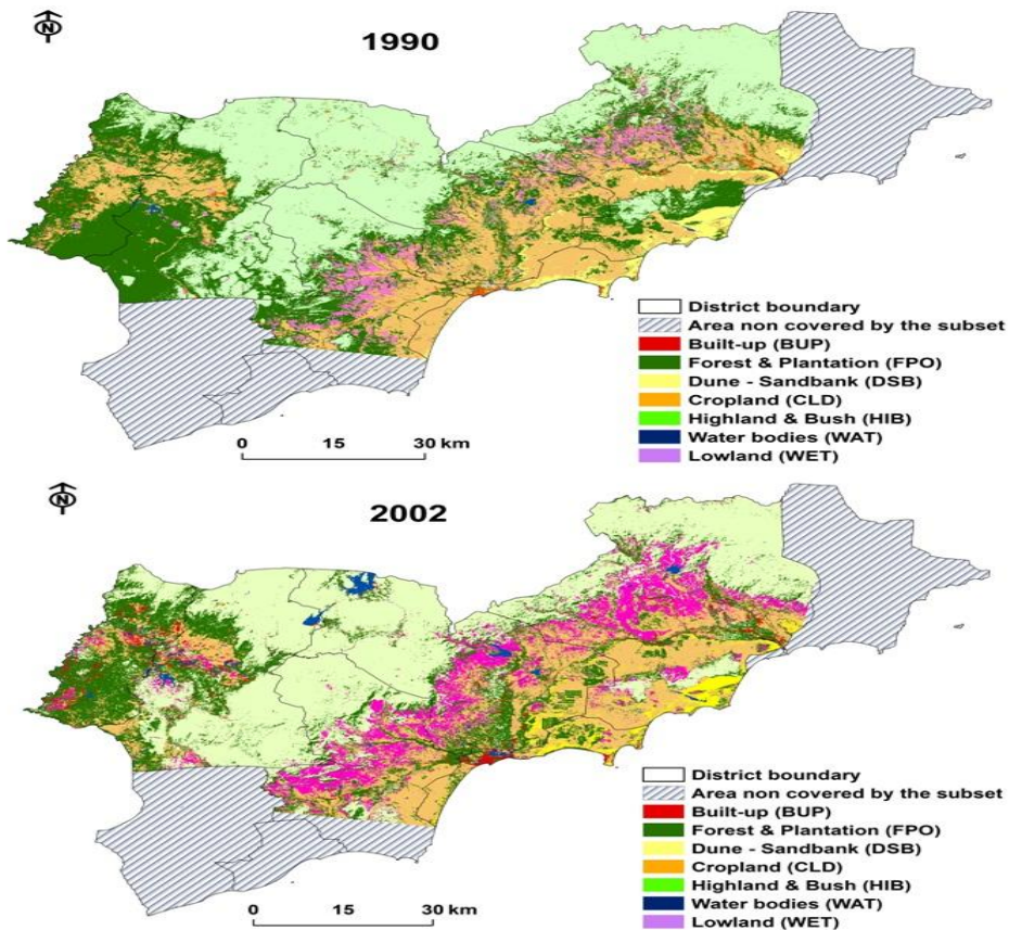
Fig-3 Land use and land cover maps (1990 and 2002) resulting from the integration of supervised classification and visual interpretation
