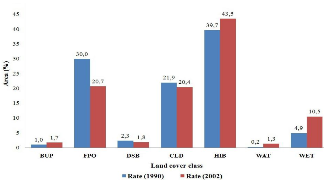
Fig-2 Area percentage of each land cover class resulting from the classified images (1990 and 2002)
