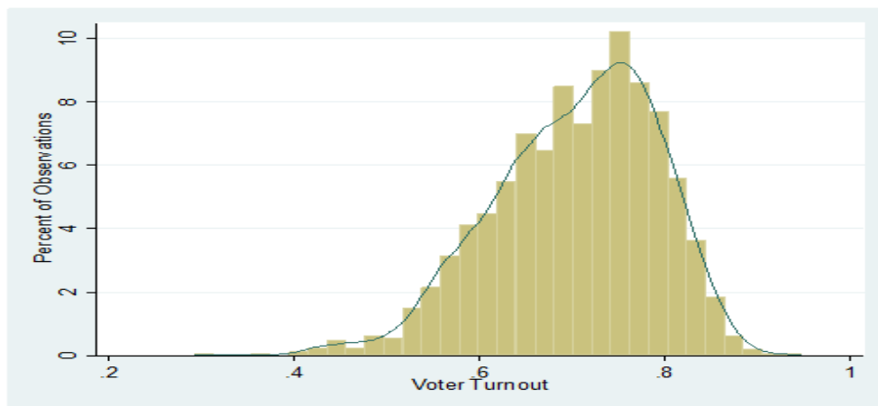
Fig-1. Histogram of Voter Turnout 2008-2013
