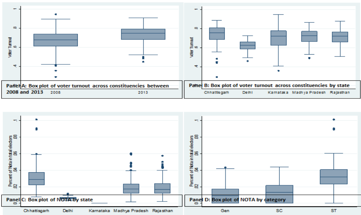
Fig-2. Box Plots of Voter Turnout and NOTA votes
